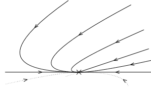
Fig. 33.10. The phase portrait near (2, 0) .
