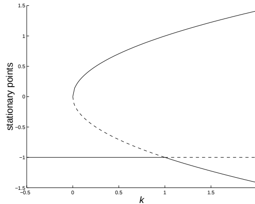
Fig. 7.16. The bifurcation diagram for the equation \dot{x} = -(1+x)(x^2 - k) [solid/dashed lines indicate stable/unstable stationary points]. There is a saddle-node bifurcation near x = 0 as k passes through zero, and a transcritical bifurcation near x = -1 and k passes through one.
