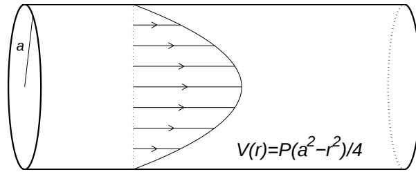
Fig. 5.1. The quadratic velocity profile in a circular pipe.
