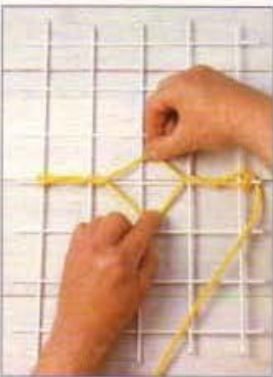
4 Twist the two parts of the lashing together, until most of the slack is removed. Find the centre of the twist.
