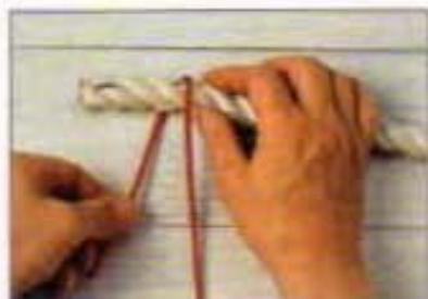
1 Lead the working end of a short length of cord or twine, from front to back, over the object to be seized.
