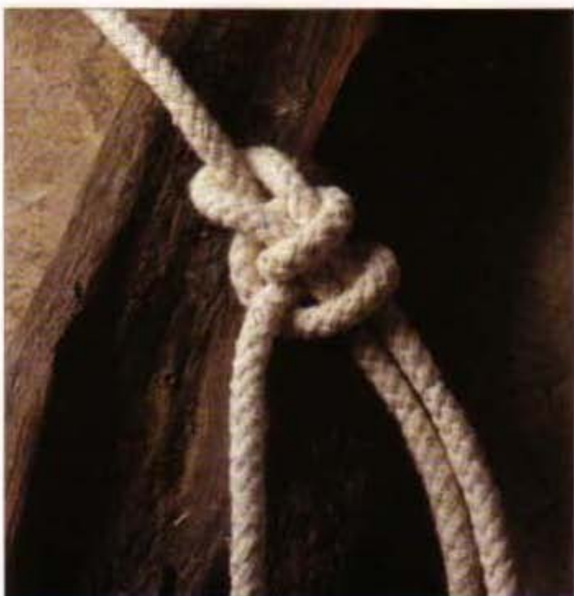
4 Pass the working end up through this second loop as well.
