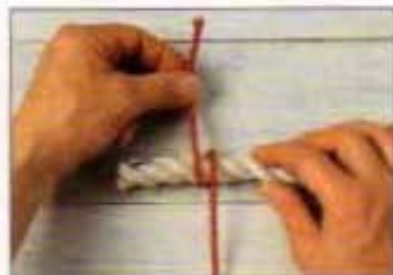
2 Lift the working end so as to complete a full turn.
