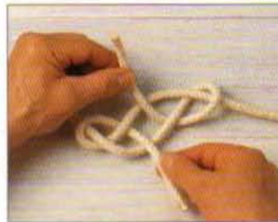
5 Turn the half-completed knot end-for-end and tie an identical crossing knot with the other working end. Work the knot tight, so that both ends protrude together from the same side of the knot.
