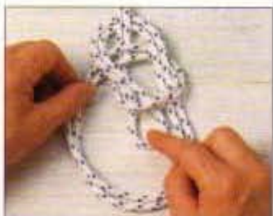
7 Tuck the bight down (from front to back) through the knot, forming the third loop. Grasp all six loop legs in one hand, holding the two standing parts in the other, and pull apart to tighten. If one of the standing parts is short, tie it to its partner with a double overhand knot.
