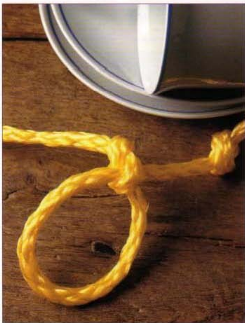
1 With the working end of a rope, make a clockwise underhand loop.
