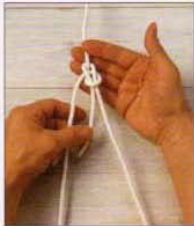
4 Finally, tie a bowline in the shorter end to the standing part.
