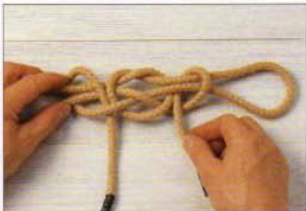
9 Tuck the working end through its own loop from back to front to tie another half hitch.
