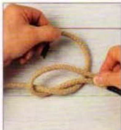
3 Lead the working end around the back of both parts of the bight.
